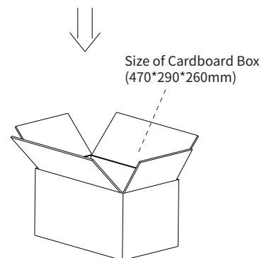
3. Place 40mm thick EPEs at the bottom and four sides of the cardboard box
