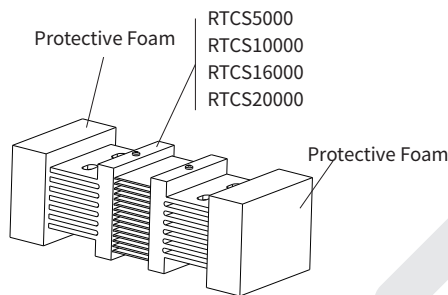
1. Cover the fins at both ends of the shunt with protective foams.
